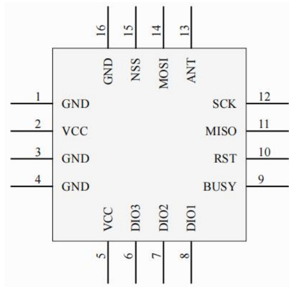
Figure 5-1 Pin definition
