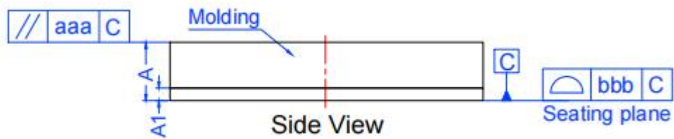
Figure 4-2 Side view
